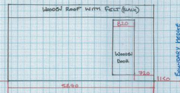
PLAN (B) 1:50 SCALE
